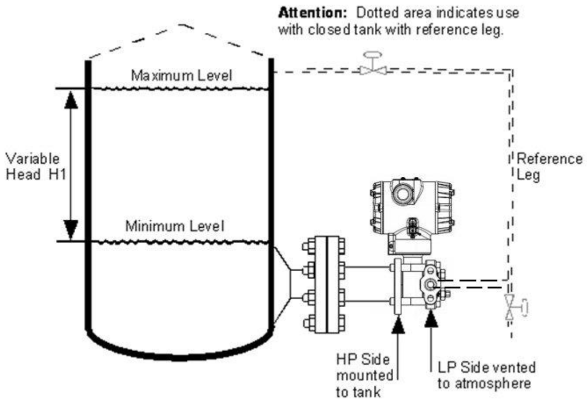
Figure 3 – Typical mounting for flange mounted level transmitter
