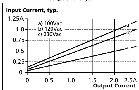
Fig. 3-3 Input current vs. output load at 24V output voltage
